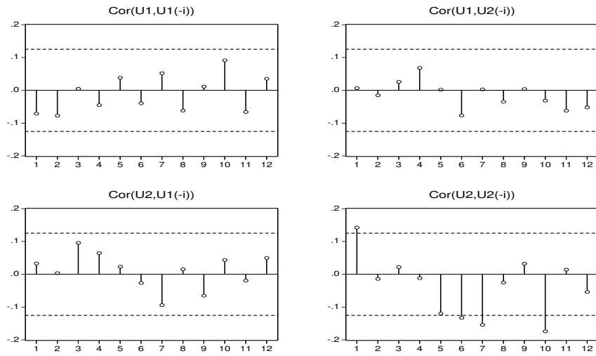
Figure 6: Cross-autocorrelogram for the VAR(1) residuals. The dashed line-bounds indicate \pm 2 \times (standard deviations), which correspond to an approximate 95% confidence bound.
