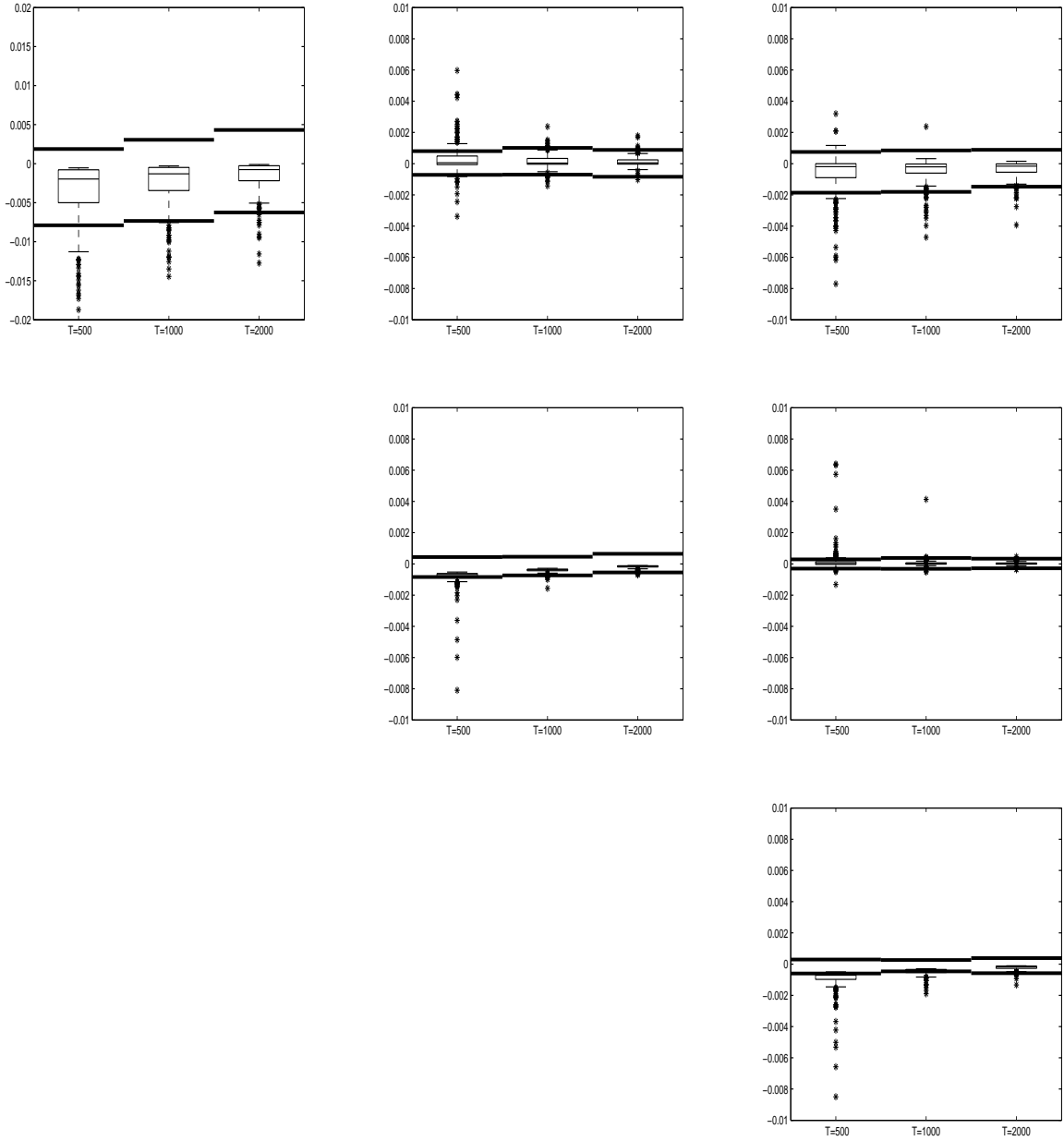
Figure 3: The boxplots based on 250 values of the entries of the scaled difference of the covariance matrices given at (10). The lengths of the series Z_t and \tilde{Z}_t were 500, 1000, 2000. The thick lines represent the upper and lower quartiles of (11).
