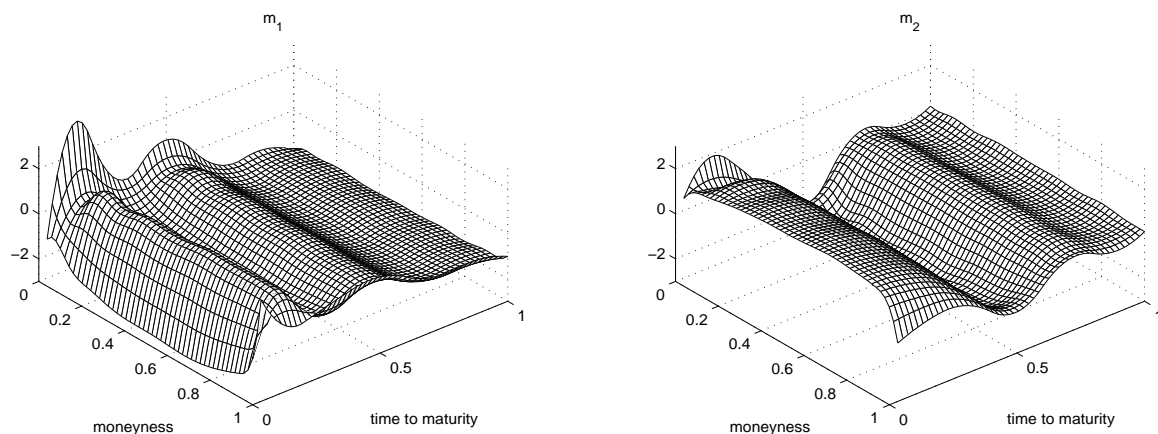
Figure 4: The estimated factor functions for the ODAX IV data from 20040701 to 20050629.
