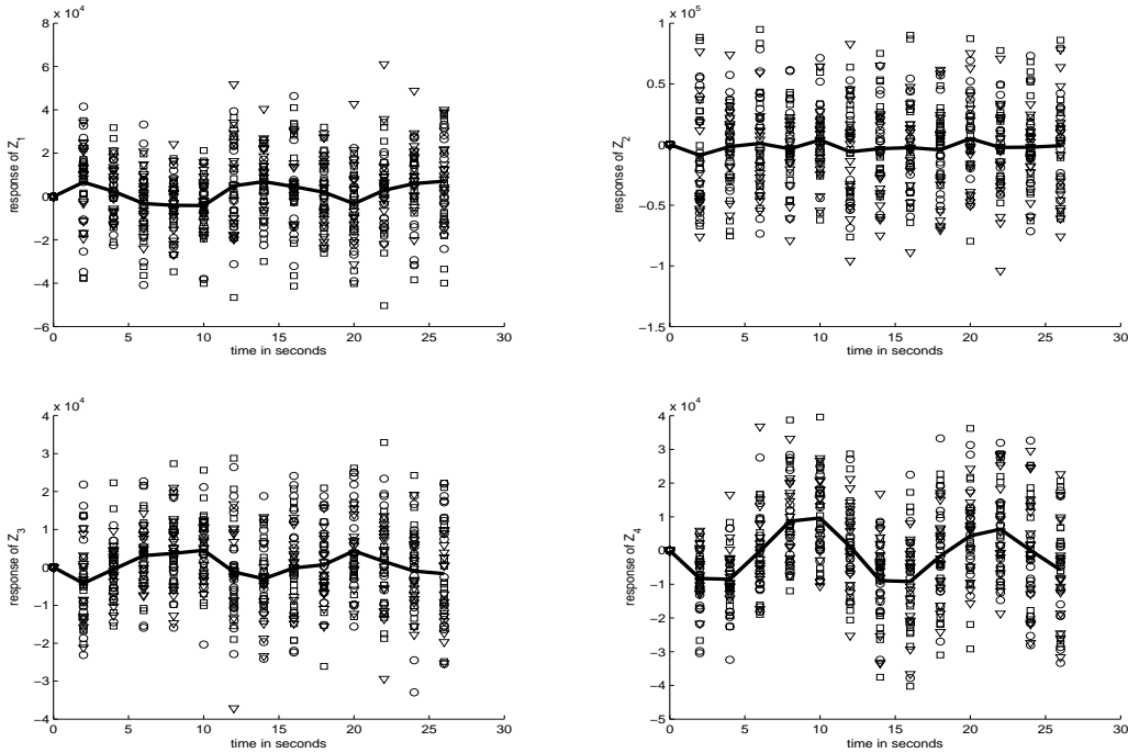
Figure 10: The responses of \hat{Z}_{t,l} to the stimuli.
