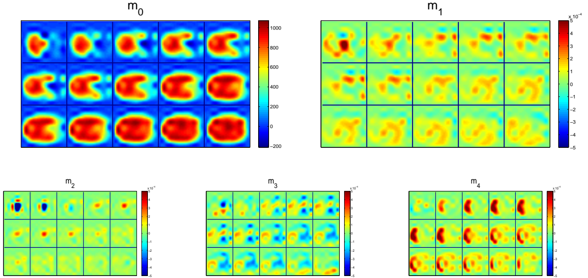
Figure 8: The estimated functions \widehat{m}_l for the fMRI signals.
