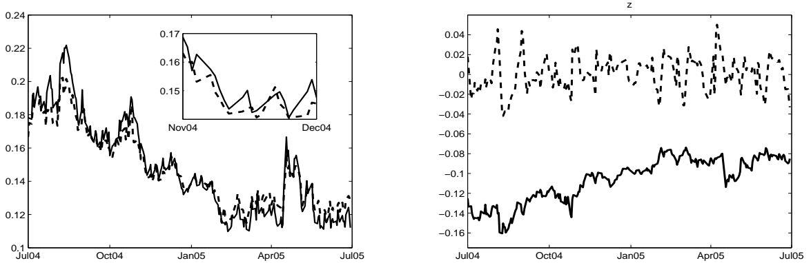
Figure 5: Left panel: VIX from 20040701 to 20050629 (solid) and the dynamics of the corresponding IV given by the sub-model \hat{m}_0 + \hat{Z}_{t,1}\hat{m}_1 (dashed). Right panel: The obtained time series \hat{Z}_t on the ODAX IV data from 20040701 to 20050629. The solid line represents \hat{Z}_{t,1} , the dashed line \hat{Z}_{t,2} .
