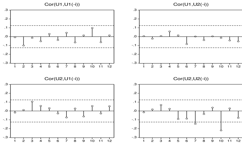
Figure 7: Cross-autocorrelogram for the VAR(2) residuals. The dashed line-bounds indicate \pm 2 \times (standard deviations), which correspond to an approximate 95% confidence bound.
